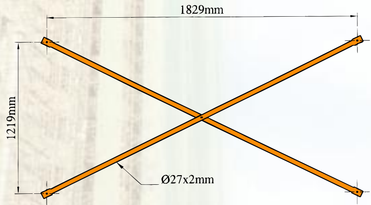
CROSS BRACE
