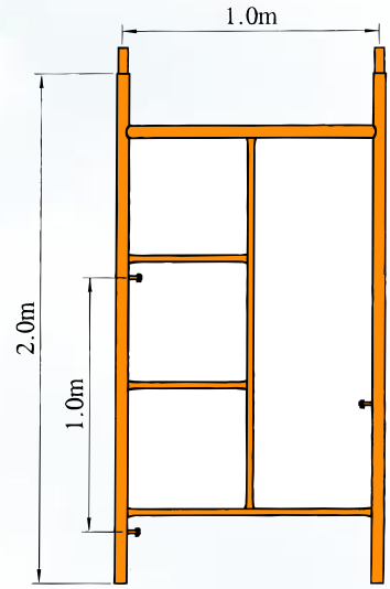
SINGLE LADDER FRAME
