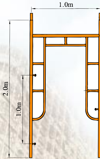
DOUBLE LADDER FRAME
