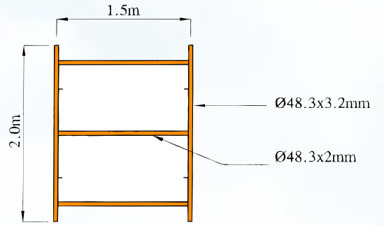
VERTICAL FRAME
