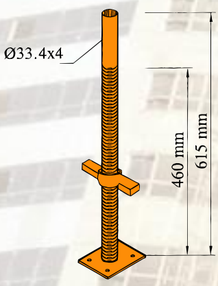
BASE JACK
