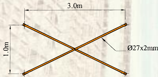
DIAGONAL BRACE
