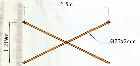
CROSS BRACE
