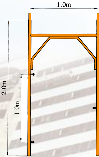
ITALIAN FRAME
