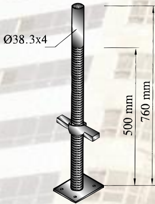
BASE JACK
